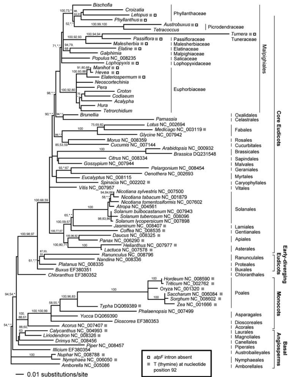
Fig. 4 Phylogenetic tree of the 76-taxon atpF dataset. Tree shown is from a ML analysis with -\ln L = 8741.21059 . Number series above or below branches indicate support from BI, ML, and MP analyses, respectively; single numbers indicate all 3 values are identical. Asterisk indicates <50% support in that analysis. Intron absence is indicated with an open square ; all other taxa possess the atpF intron. A filled gray square indicates the presence of a thymine at nucleotide 92; all other taxa possess a cytosine at that site, which is potentially RNA edited as a C-U conversion. GenBank numbers are indicated for published data, all other taxa are newly generated (see Appendix )
