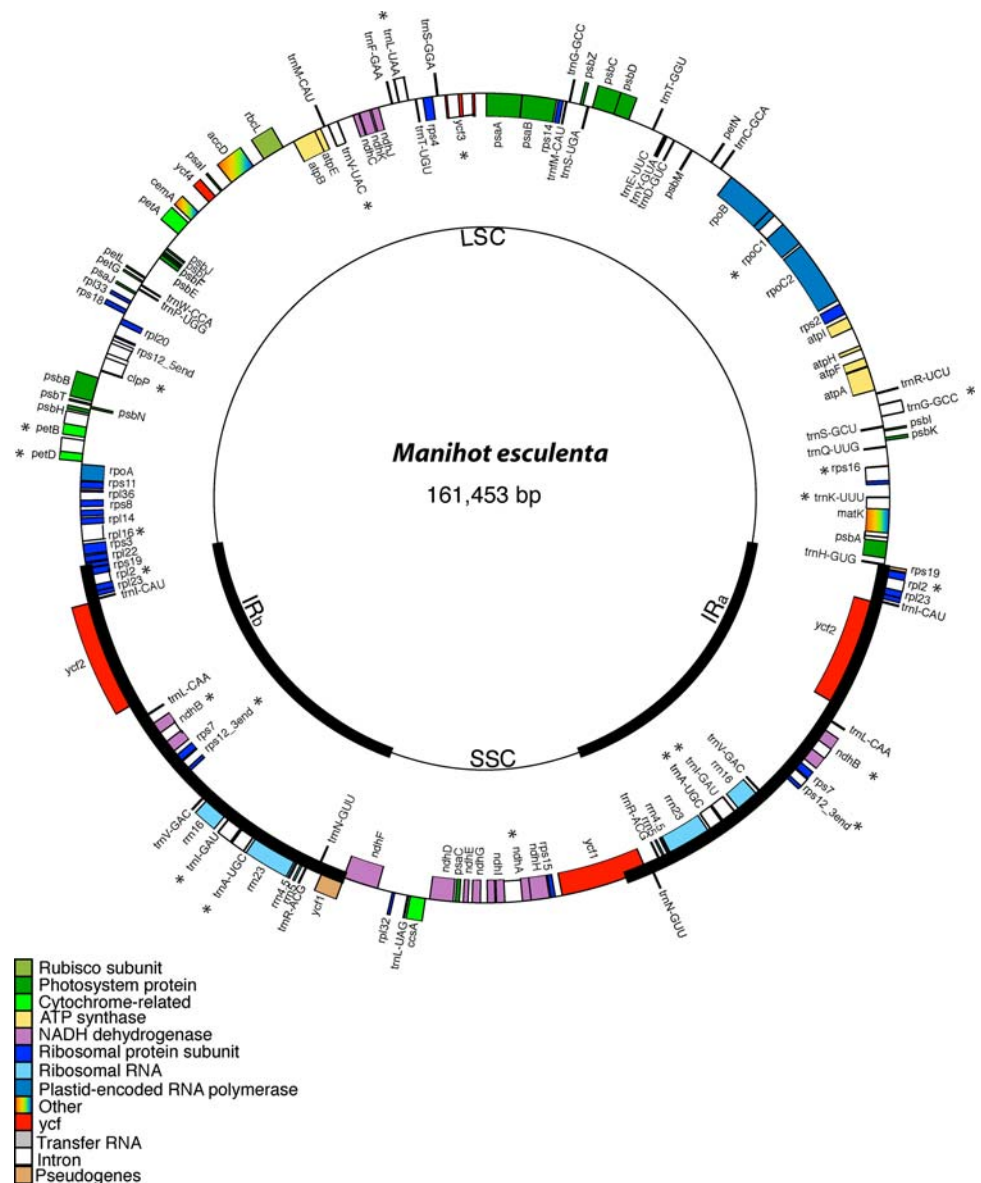
Fig. 1 Map of the M. esculenta plastid genome represented in its circular monomeric form. Large and small single copy regions ( LSC , SSC ) are separated by the inverted repeats ( IRa and IRb , 26,954 bp, respectively). Genes illustrated inside the circle are transcribed in the clockwise direction and genes illustrated outside the circle are transcribed in the counter-clockwise direction. Split genes or genes with introns are marked with asterisks
